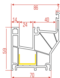
Marco Monorriel Corredera
