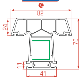
Mullion Profile
