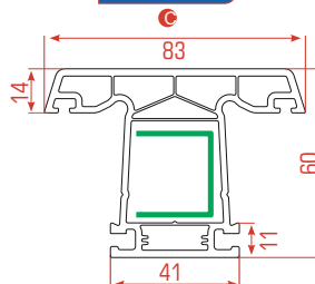
Mullion Profile
