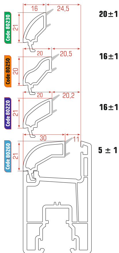
Sliding System
