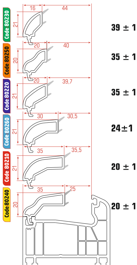
S76X6
