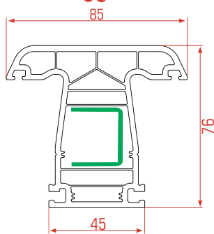
Mullion Profile
