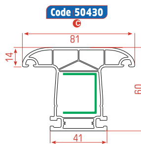
Mullion Profile
