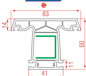
Mullion Profile
