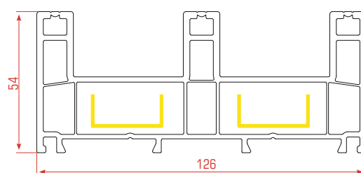
Marco Corredera Triple Riel
