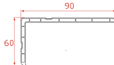
Angle PVC Profile
