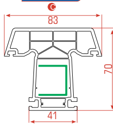
Mullion Profile
